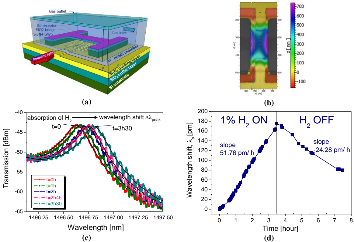
Fig. 2. (a) 3D schematic of the mechano-optical sensor structure with a PDMS chamber serving as a reaction environment for H 2 sensing; (b) top view image of the device attained using a white-light interferometer, showing an initial up-bending of ~500 nm at the center of the micro-bridge; (c) transmission curves of the device in response to the absorption; (d) wavelength shift \Delta\lambda_p versus reaction time.
