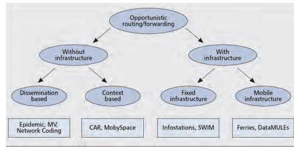
Fig. 2. Taxonomy of opportunistic routing [12]
