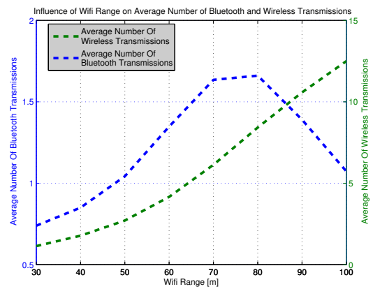
Fig. 7. Bluetooth and WiFi's contribution with WiFi range
