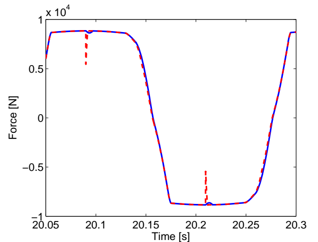
Figure 10: Damper force vs time for well (solid) and poorly (dashed) designed circuits)
