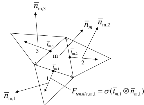
Figure 1: Surface tension force exerted by three neighbouring surface elements on the central surface element.
