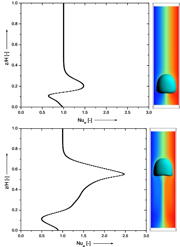
Figure 6: Profile of the instantaneous Nusselt number (left) and corresponding bubble position (right) for t=0.05 s (top) and t=0.30 s (bottom).
