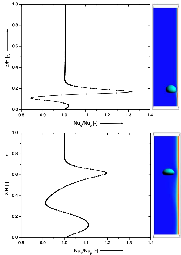
Figure 4: Profile of the instantaneous dimensionless heat transfer coefficient (left) and corresponding bubble position (right) for t=0.05 s (top) and t=0.30 s (bottom).
