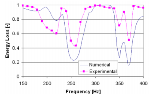
Figure 4 : Experimental and numerical results
