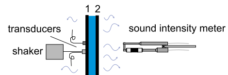
Figure 3 : Intensity measurements on double walls
