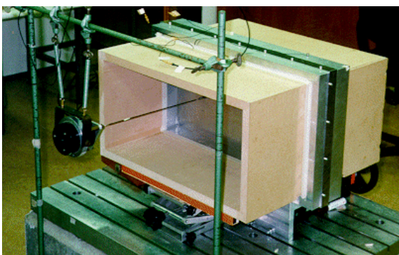
Figure 2 : Experimental setup
