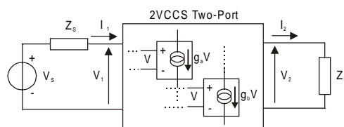
Fig.4: 2VCCS two-port model.
