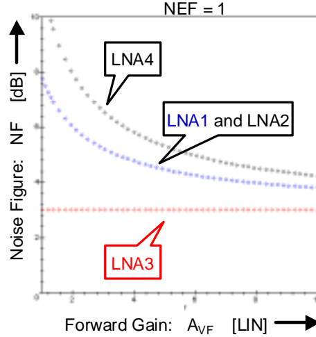
Fig. 6: LNA Noise figure F_{dB}=10\text{Log}_{10}(F) .
