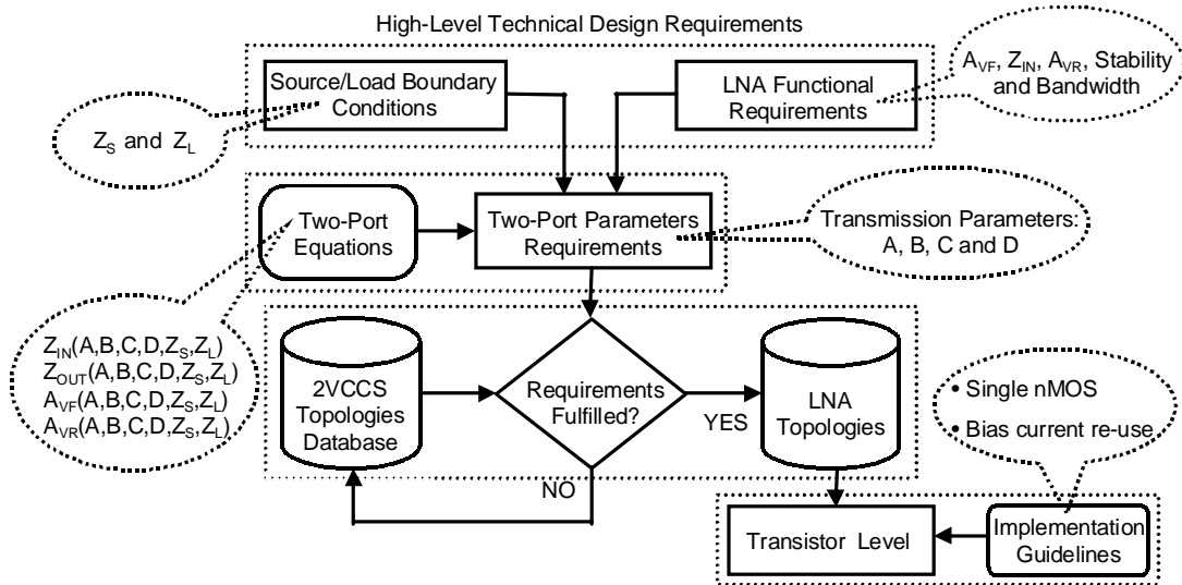
Fig.3: Block diagram of the generation methodology.
