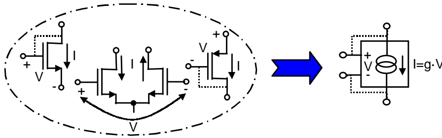
Fig.1: VCCS representation of simple MOS circuits.
