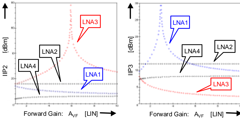
Fig.7: IIP2 dBm and IIP3 dBm versus the forward gain A_{VF,V} upon \min P_{LNA,min} .
