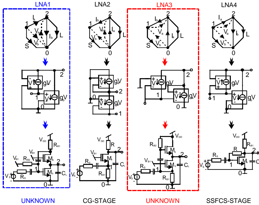
Fig.5: Graph, VCCS and nMOST representation of the 4 selected 2VCCS LNAs.
