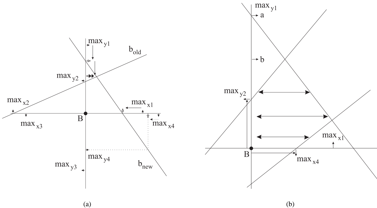
Figure 2. Principle of the bookkeeping and updating. (a) Keeping track of the maximum x and y values per quadrant around a border pixel. (b) Updating along scan lines: bisection lines determine start and end points on them.
