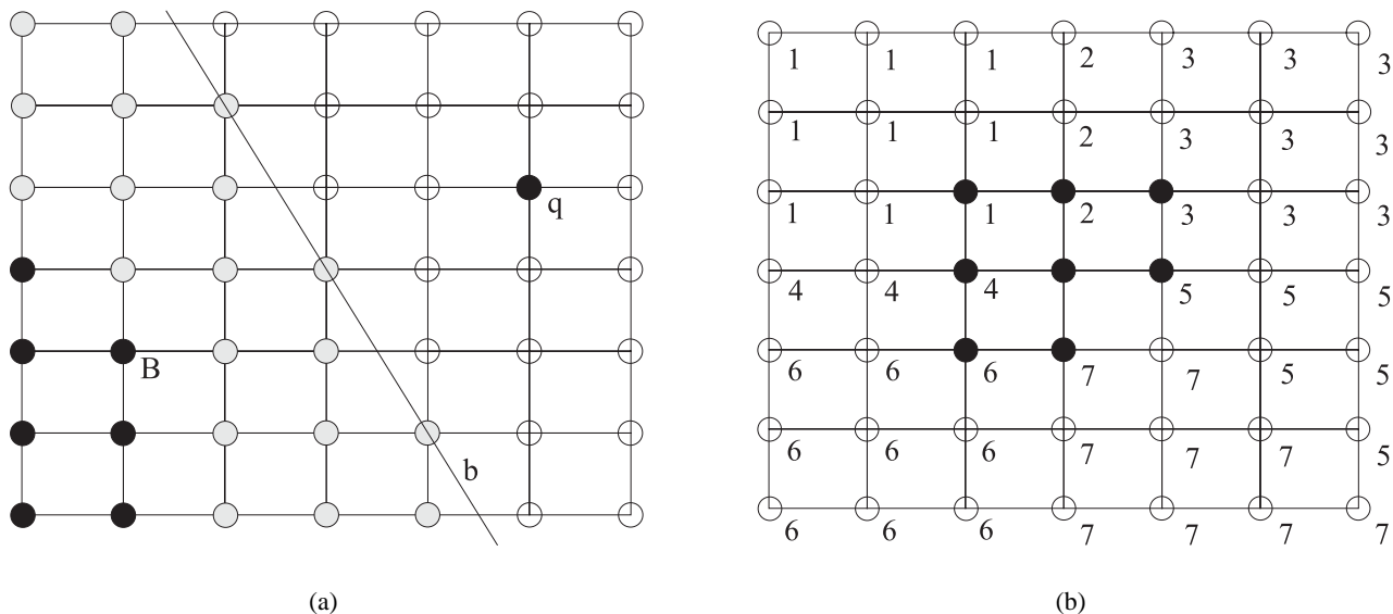
Figure 1. Principle of limiting the number of background pixels to update. (a) Only pixels on and to the left of the bisection line b between a border pixel B and an object pixel q have to be updated. (b) An example showing that each background pixel has to be updated only once. Each background pixel is labeled by the border pixel which updates it.
