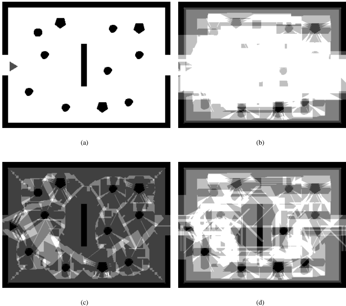
Figure 3. The number of updates used for several settings of the search parameters. Pixels with 0 updates are indicated in black, pixels with 4 or more updates in white. (a) An input image with 76800 pixels, 13942 object pixels and 1725 border pixels. (b) Too little searching resulting in 290771 updates and an execution time of 5.7 ms. (c) Too much searching resulting in 86487 updates and 8.4 ms execution time. (d) Optimal searching resulting in 179373 updates and 4.5 ms execution time.
