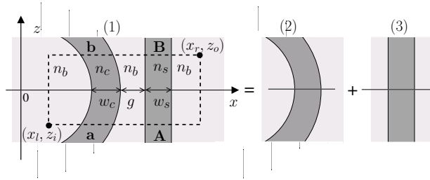
Figure 2: CMT setting for bent-straight waveguide couplers. The coupler is defined in the region [x_l, x_r] \times [z_i, z_o] . The external segments of the bent waveguide and the straight waveguide constitute the port connections. It is assumed that outside the coupler there is negligible interaction between the waveguides.
