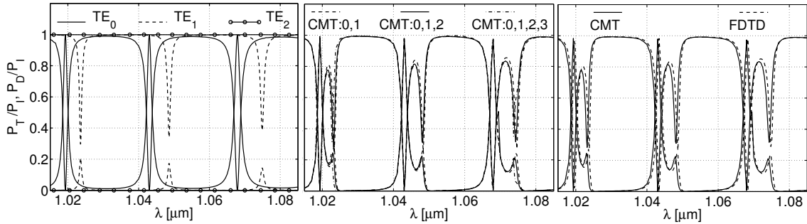
Figure 3: TE power spectrum for a 2D disk microresonator. Left : CMT with only a single (one of TE_0, TE_1 or TE_2 ) cavity mode. Middle : CMT results for two (dashed line), three (solid line) and four (dash-dotted line) cavity modes together. Right : Comparison of FDTD results and CMT results with 3 cavity modes. MR specifications: n_c = n_s = 1.5 , n_b = 1.0 , w_c = 0 \mu\text{m} (disk), w_s = 0.4 \mu\text{m} , R = 5 \mu\text{m} , g = 0.2 \mu\text{m} .
