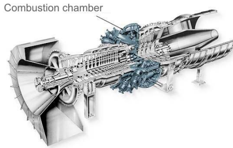
Figure 1 : Combustion chamber in Siemens gas turbine
