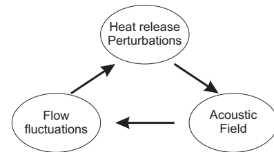
Figure 2 : Thermoacoustic feedback
