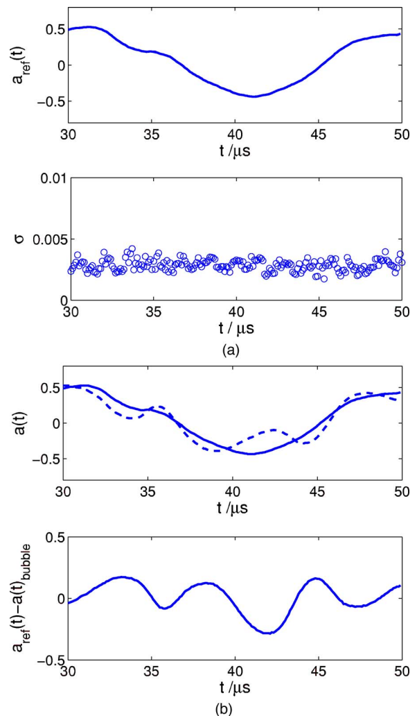
FIG. 4. (a) (Color online) The acoustical signal, a_{\text{ref}}(t) , averaged over 25 standard droplets (upper), and the corresponding standard deviation that is more than 100 times smaller (lower), showing the reproducibility of the signal. Note the 50 times enlarged scale on the y axis. (b) Upper: Acoustical signals with (dashed) and without (solid) an air bubble present in the ink channel. The lower panel shows the difference of these two signals.
