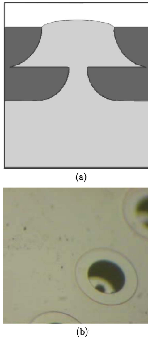
FIG. 12. (Color online) (a) Schematic side view of the additional nozzle plate on top of the original one. (b) Top view photograph of the setup.
