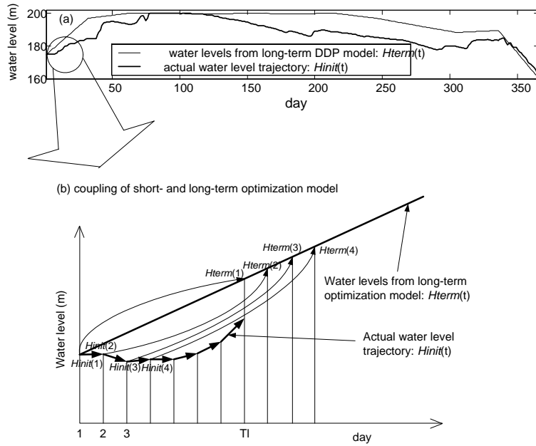
Fig. 4. Coupling of the long-term and short-term optimization models. H_{init}(t) are actual water levels which serve as the initial conditions of every short-term optimization cycle; H_{term}(t) are long-term optimization results, interpolated into daily water levels, serving as terminal conditions for each short-term optimization cycle.
