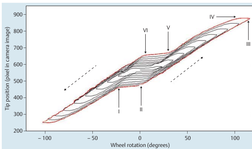
Fig. 3 Nonlinearity in the endoscope tip response. The tip is angulated in alternating up-and-down directions, with increasing bending angles. I. Cable pulling starts in neutral position. II. Tip starts bending. III. Tensed cable is released. IV. Tip starts to relax and return to straight position. V. Pulling the antagonist cable. VI. Tip follows the antagonist cable.
