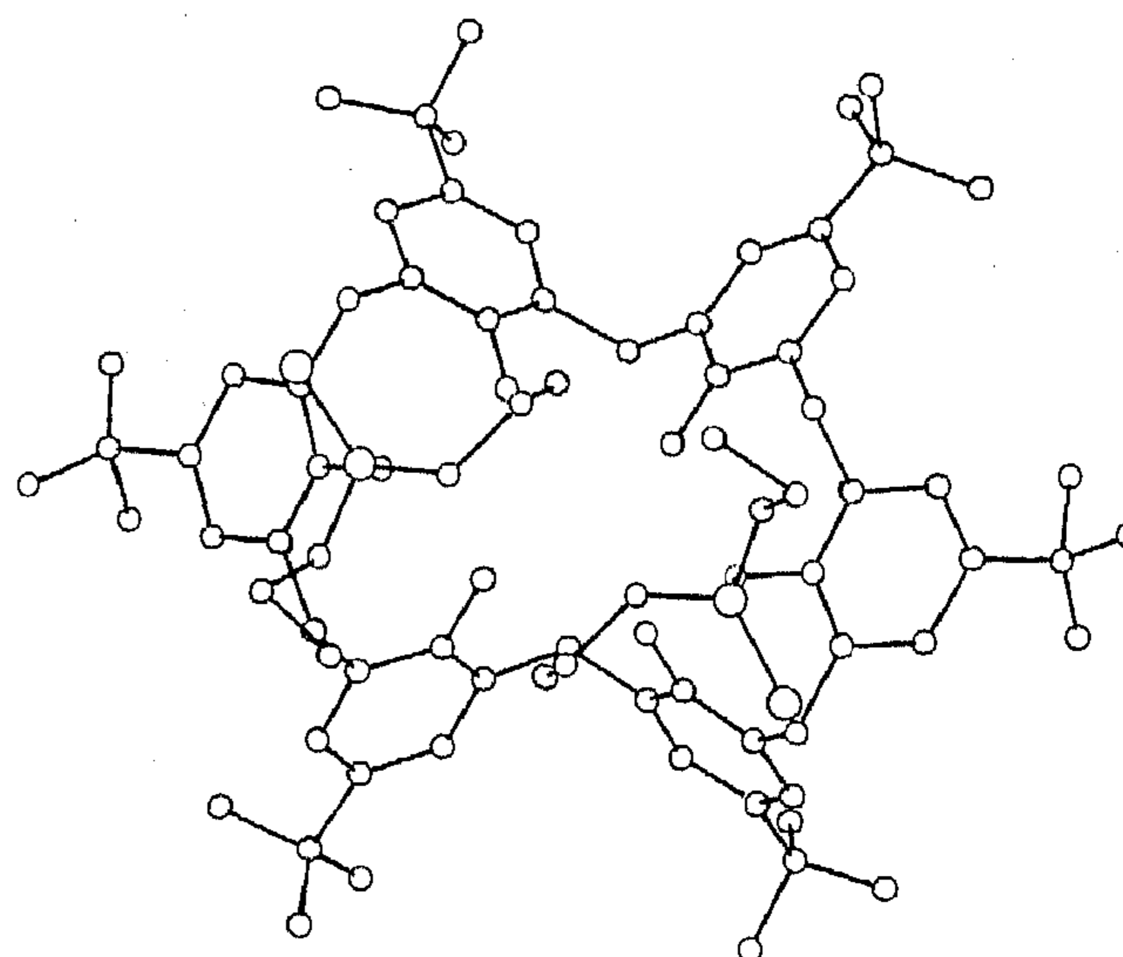
Fig. 1 Solid-state structure of compound 7
