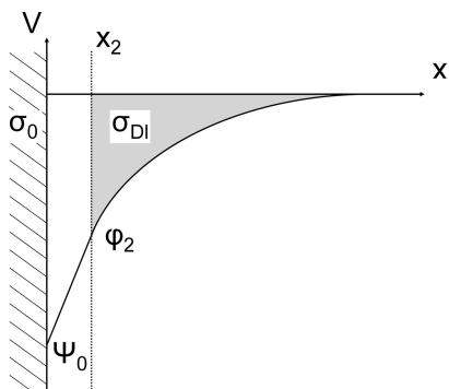
Figure 5. Schematic representation of potential V versus the distance x from the silicon oxide wall. \Psi_0 is the potential at the wall. x_2 is the position of the Stern plane, the plane of closest approach of ions toward the surface, having the potential \phi_2 . The region from the wall to the Stern plane is called the Stern layer. \sigma_0 (eqs 8 and 13) indicates the surface charge per m^2 from deprotonated silanol groups at x = 0 . \sigma_{DL} is the countercharge to \sigma_0 per m^2 (eq 11), composed of ions located in the area beyond the Stern plane, the so-called diffuse part of the double layer (gray region).
