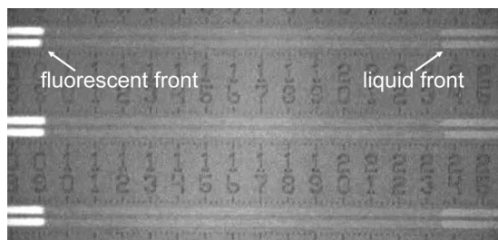
Figure 1. Typical image of fluorescence observed in nanochannels during filling. In this experiment, (experiment no. 1 of Table 1, screenshot of Movie S-1), the partial filling of parallel channels, 20 \mu\text{m} wide and 40.5 nm deep, taken at t = 5 s, are shown. From left to right the channel is filling from the reservoir, which is outside the image shown. Fluorescence is observed in the filled zone, from x = 0 to x = 0.92 mm, but not in the zone from x = 0.92 mm to 2.36 mm.
