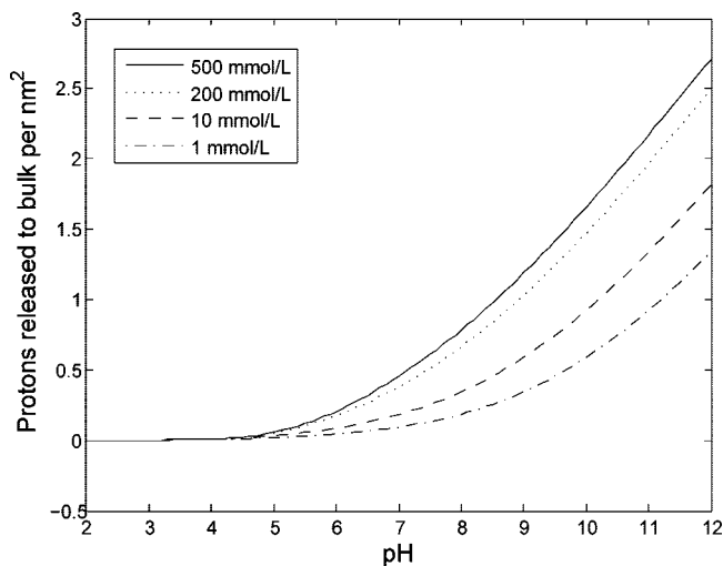
Figure 6. Theoretical amount of deprotonated silanol groups per \text{nm}^2 as a function of pH. The different curves, belonging to 1, 10, 200, and 500 mmol/L of KCl, show the effect of the ionic strength on proton release, with more salt inducing a higher release, which will be observed as a shorter fluorescent zone.
