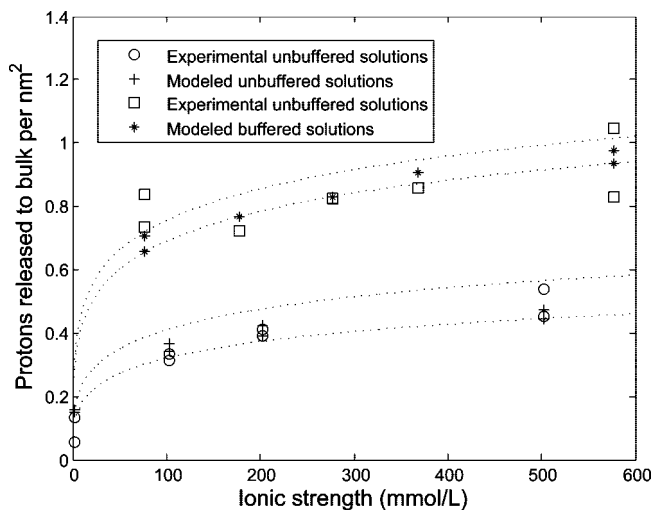
Figure 7. Results of the experiments, N_{\text{H}_{\text{exp}}^+} fitted with the model, N_{\text{H}_{\text{theory}}^+} . Fits were made using the input and fitting parameters from Tables 1 and 2, with the dissociation constants \text{p}K_{\text{a}1} = 6.77 and \text{p}K_{\text{a}2} = -1.90 and therefore a \text{pH}_{\text{pzc}} = 2.44 . A value of C_{\text{Stern}} = 2.30 \text{ F/m}^2 led to the optimal fit with R^2 = 0.93 for the unbuffered solutions and R^2 = 0.37 for buffered solutions. The data point for the buffered solution at an ionic strength of 386 mmol/L has a buffer strength of 1 mol/L, the others 0.2 mol/L. The dashed lines indicate the modeled values corresponding to the extremes of pH in the introduced solutions, from top to bottom, \text{pH} = 8.6 , \text{pH} = 8.4 , \text{pH} = 7.4 , and \text{pH} = 7.0 .
