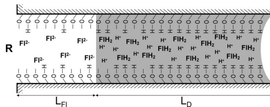
Figure 3. Axial cross-section of a filling nanochannel. R indicates the reservoir from which the nanochannel is filled. L_{\text{FI}} and L_{\text{D}} correspond to the fluorescent and dark zone of the channel, respectively. In the fluorescent zone the pH is that of the introduced solution where fluorescein is present mainly as doubly charged anions ( \text{FI}^{2-} ). The fluid in the dark zone contains an excess of protons, with \text{pH} = \text{pH}_{\text{pzc}} and fluorescein is mainly present as the uncharged fluorescein molecule ( \text{FIH}_2 ), having negligible fluorescence.
