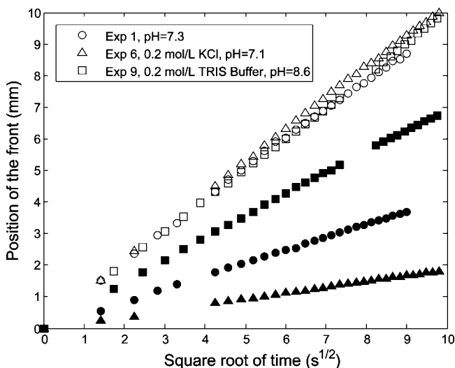
Figure 4. Position of the meniscus (empty symbols) and the fluorescent front (filled symbols) versus the square root of time for experiments 1, 6, and 9. All graphs could be linearly fitted using a least-squares method with a value of R^2 > 0.99 .
