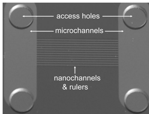
Figure 2. Chip layout seen from the top. Vertically, the microchannels connecting the two pairs of access holes can be seen and between them the rulers positioned along the nanochannels are visible. The nanochannels are 50 nm deep and 20 \mu\text{m} wide, the microchannels are 20 \mu\text{m} deep, 15 mm long, and 4 mm wide.
