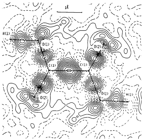
Fig. 4. Experimental difference electron density in the plane of the oxalic acid molecule. Contours are drawn at intervals of 0.05 \text{ e \AA}^{-3} ; zero and negative contours dashed.
