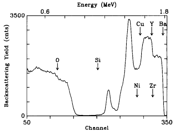
Fig. 5. RBS spectrum of sample 3. The laser-pulse frequency was set to 10 Hz and the deposition time of the YBa_2Cu_3O_{7-\delta} layer was 6 min.
