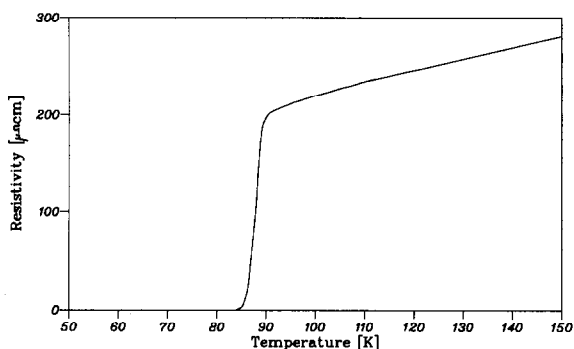
Fig. 2. \rho-T curve of YBa_2Cu_3O_{7-\delta} layer (sample 4), deposited on a Si substrate with a NiSi_2/ZrO_2 buffer layer using laser ablation.
