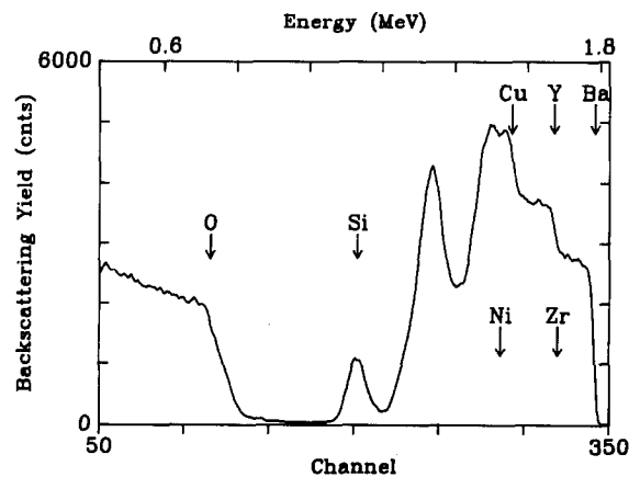
Fig. 7. RBS spectrum of sample 4. The laser-pulse frequency was set to 2 Hz and the deposition time of the \text{YBa}_2\text{Cu}_3\text{O}_{7-\delta} layer was 35 min.
