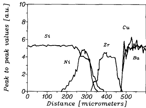
Fig. 8. Line profiles on crater edge in sample 3. See also fig. 1. The laser-pulse frequency was set to 10 Hz and the deposition time of the \text{YBa}_2\text{Cu}_3\text{O}_{7-\delta} layer was 6 min.
