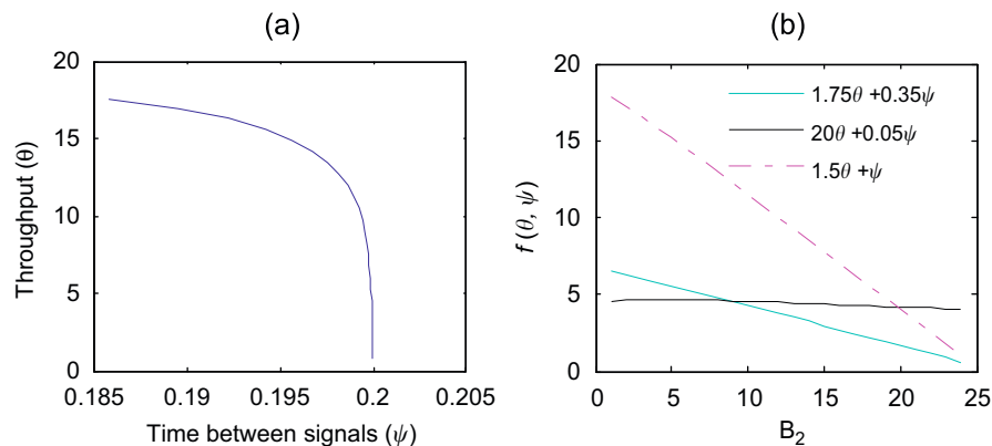
Fig. 9. Trade-off between throughput \vartheta (in Mbit/s) and time between signals \psi (in s) for higher traffic aggregation model.
