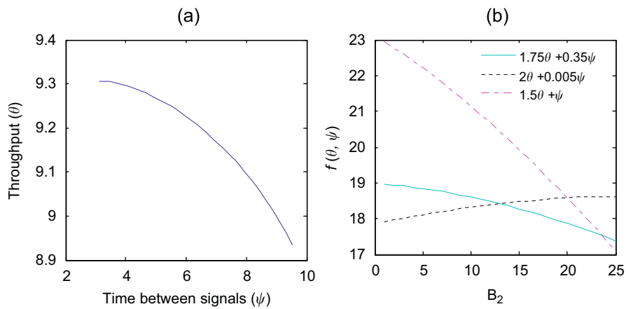
Fig. 7. Trade-off between throughput \vartheta (in Mbit/s) and time between signals \psi (streaming traffic, in s).
