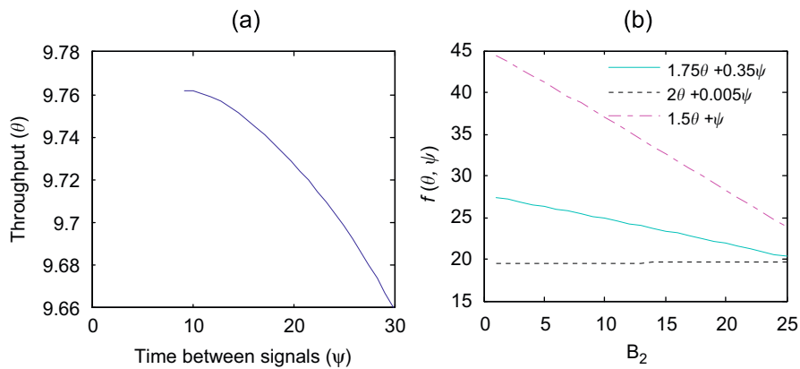
Fig. 8. Trade-off between throughput \vartheta (in Mbit/s) and time between signals \psi (elastic traffic, in s).
