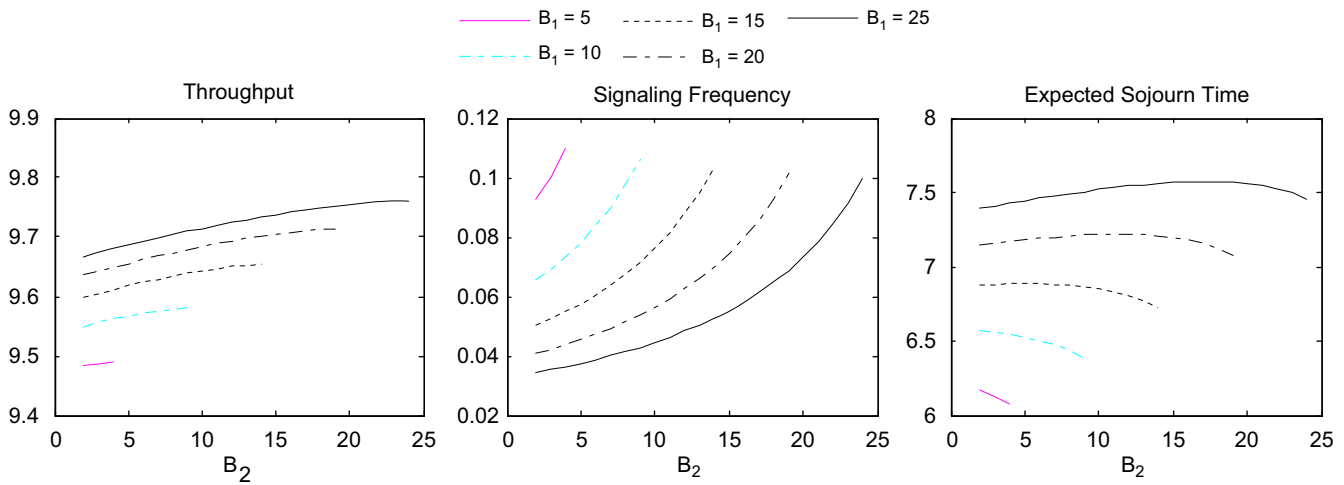
Fig. 5. Effect of thresholds on elastic traffic (throughput in Mbit/s, the signalling frequency in s^{-1} , and the expected delay in s).
