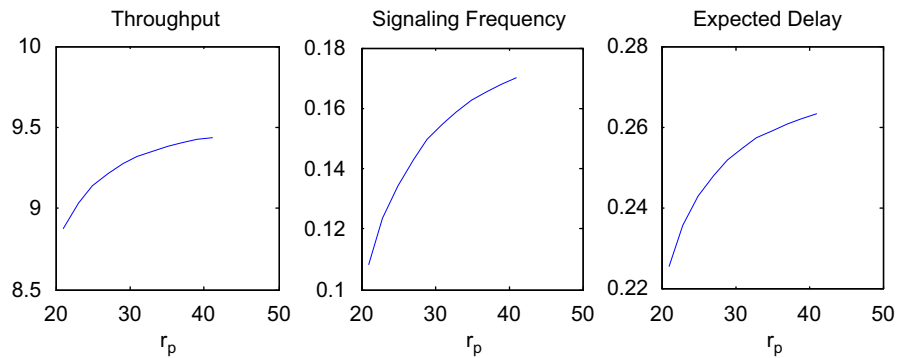
Fig. 3. Effect of transmission rate r_p on streaming traffic; B_1 = 25 and B_2 = 10 (throughput in Mbit/s, the signalling frequency in s^{-1} , and the expected delay in s).
