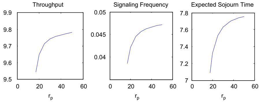
Fig. 6. Effect of varying r_p and p_1 while keeping their ratio fixed at r_p/p_1 = 25 (throughput in Mbit/s, the signalling frequency in s^{-1} , and the expected delay in s).
