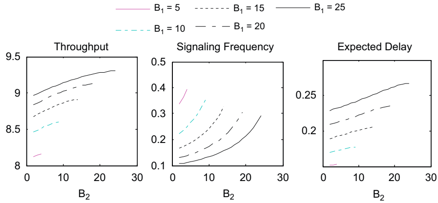
Fig. 2. Effect of thresholds on streaming traffic (throughput in Mbit/s, the signalling frequency in s^{-1} , and the expected delay in s).
