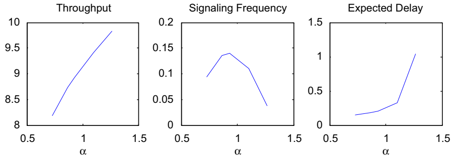
Fig. 4. Effect of multiplying r_p and r_m by factor \alpha ( \alpha is such that the stability condition is satisfied); B_1 = 25 and B_2 = 10 (throughput in Mbit/s, the signalling frequency in s^{-1} , and the expected delay in s).
