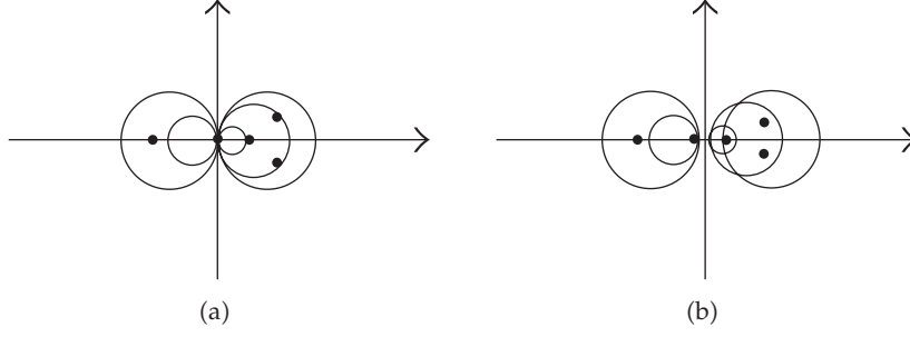
Figure 2: Eigenvalues in the complex plane. (a) Eigenvalues of -R_A^{-1}\check{Q} ; (b) eigenvalues of -R_A^{-1}(\check{Q} - \epsilon D) . In this example N = 5 , and there are 3 up-states and 2 down-states.
