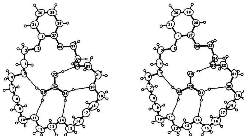
Figure 1. Stereoscopic view of the benzo-27-crown-9.UrHClO 4 (1:1) complex, showing atom numbering. The perchlorate ion (numbered O37-O40) is omitted.
