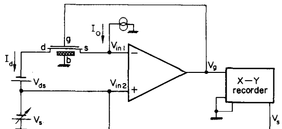
Fig. 2. Measurement circuit. The current source I_o and the voltage source V_{ds} can be adjusted to attain the desired turn-on condition ( G = 10^{-7} mho) in the MOST. The voltage V_s is the independent variable.
