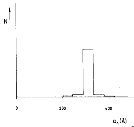
Figure 4. Number distribution function of the polystyrene latex.
