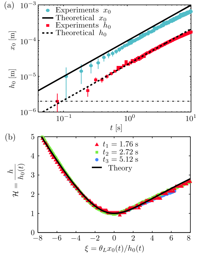
FIG. 3 (color online). Asymmetric coalescence. (a) Horizontal and vertical position of the meniscus bridge, x_0(t) and h_0(t) , for asymmetric drops ( \theta_L = 46^\circ , \theta_R = 13^\circ , viscosity \eta = 12.2 \text{ Pa} \cdot \text{s} ). Blue (●) and red (■) markers are experimental data for x_0 and h_0 , respectively. Solid and dashed lines are the predictions from the similarity solutions. (b) Rescaled experimental profiles at different times, \mathcal{H} = h(x, t)/h_0(t) versus \xi = x_0\theta_L/h_0(t) . The collapse reveals self-similar dynamics at the early stage of coalescence. The solid line is the similarity solution predicted by our analysis.
