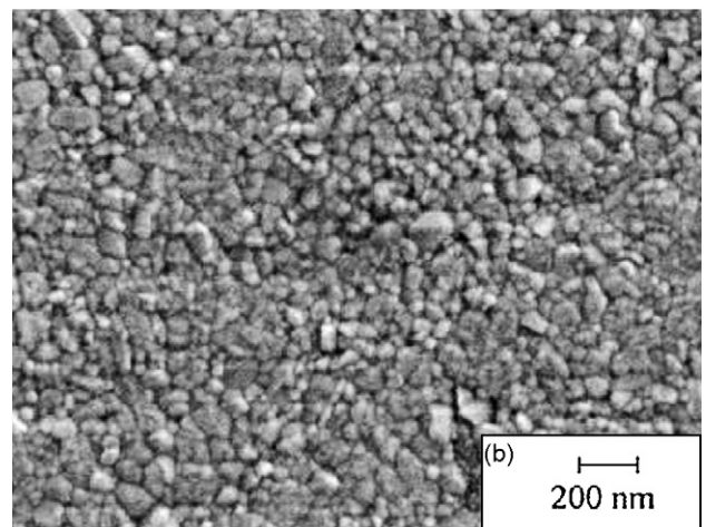
Fig. 7. SEM picture of a polished and thermally etched 8 mol% CuO-doped 3Y-TZP nano-powder compact; (a) after sintering for 2 h at 1130 °C (heating rate 15 °C/min); (b) after sintering for 20 h at 960 °C (heating rate 20 °C/min).
