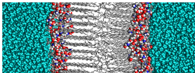
FIGURE 4 Snapshot of the ceramide bilayer in the gel phase at 323 K. The ceramide tails of both layers are packed in a hexagonal arrangement, although this is not apparent for the right leaflet because of a difference in orientation. The z axis runs in a direction normal to the bilayer surface. Water is cyan, ceramide carbon atoms gray, nitrogen atoms blue, oxygen atoms red, and hydrogen atoms white.
