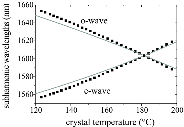
FIG. 2: Subharmonic wavelengths as a function of the crystal temperature. Symbols: measured values; solid line: theoretical tuning derived from the Sellmeier coefficients given in Ref. 19.
