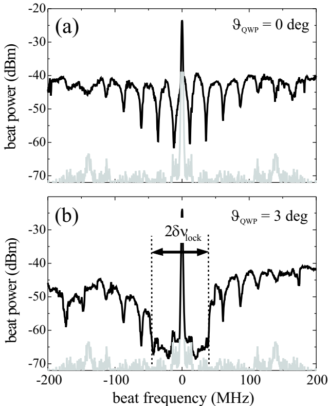
FIG. 3: Measured beat frequency spectra for a quarter-wave plate rotation angle of (a) \vartheta_{QWP} = 0 \text{ deg} and (b) \vartheta_{QWP} = 3 \text{ deg} . The beat signal power is displayed as a function of the beat frequency by the black curves, and the gray curves are the background noise level, recorded with the photodiode blocked.
