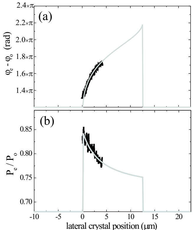
FIG. 7: (a) Phase difference and (b) Power ratio as a function of the lateral crystal position. Black trace: measured values, gray trace: theoretically calculated values.
