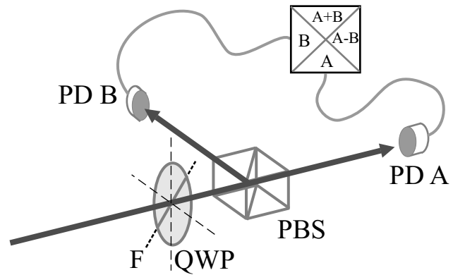
FIG. 5: Setup of the Hänsch-Couillaud-detector. QWP, quarter-wave plate with fast axis F set to 45 deg; PBS, polarizing beam splitter; PD A and PD B, photodiodes.
