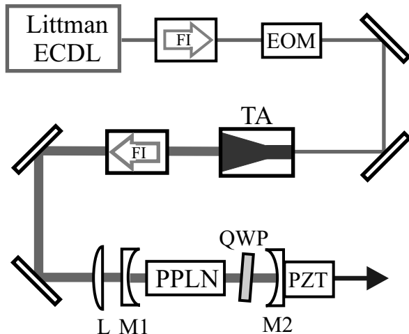
FIG. 1: Setup of the by-2 divider OPO. Littman ECDDL, Littman external cavity diode laser; FI, Faraday Isolator; EOM, electro-optic modulator for electronic stabilization of the OPO cavity length; TA, tapered amplifier; L, lens, M1, M2, cavity mirrors; PPLN, periodically poled lithium niobate crystal, QWP, quarter-wave plate; PZT, piezo transducer.
