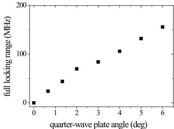
FIG. 4: Measured self-phase locking range of the OPO as a function of the QWP rotation angle.
