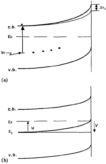
Fig. 2. (a) Schematic representation of the photovoltaic process in an n-type semiconductor with a depletion region: surface state depopulation. (b) Energy-band diagram considered in this work. All symbols are explained in the text.
