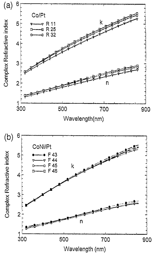
Fig. 3. Dispersion of the complex refractive index \hat{n} (= n + ik) .
