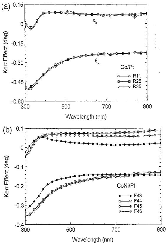
Fig. 4. Dispersion of the complex Kerr rotation \hat{\theta} (= \theta_k + i\epsilon_k) .
