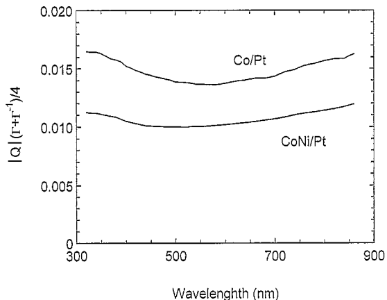
Fig. 7. Dispersion of the preferred figure-of-merit |Q|(\Gamma + \Gamma^{-1})/4 .
