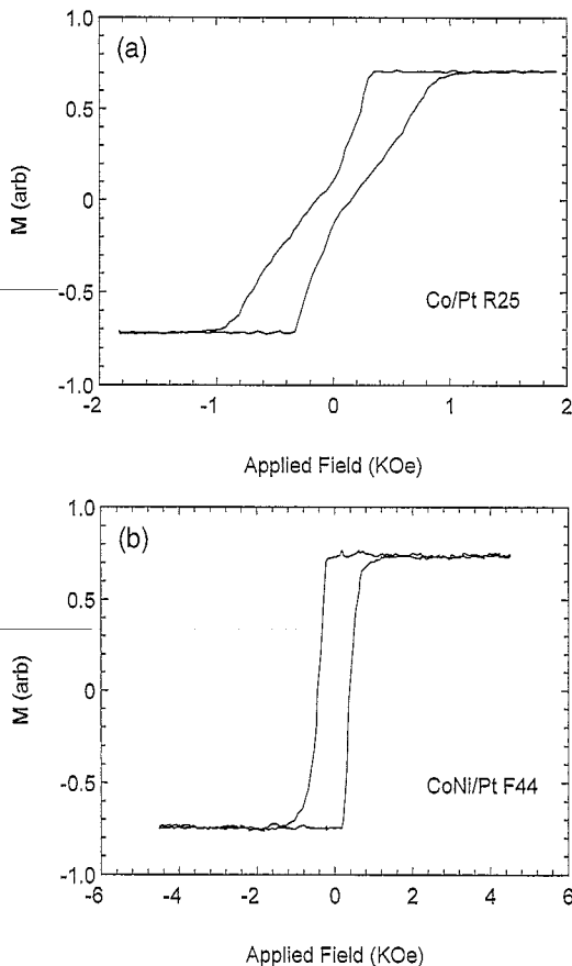
Fig. 2. M.O. hysteresis loops of (a) Co/Pt and (b) CoNi/Pt multilayer of magnetic layer thicknesses 79.5 nm and 26.9 nm, respectively. Probe wavelength = 633 nm.
