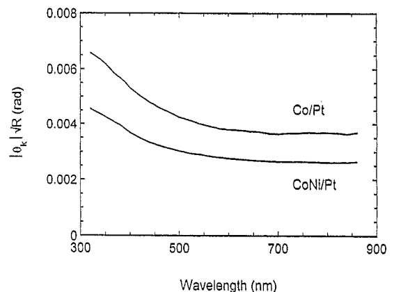
Fig. 6. Dispersion of the figure-of-merit |\hat{\theta}_k| \sqrt{R} .
