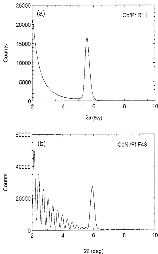
Fig. 1. Low angle X-ray diffraction patterns for (a) Co/Pt and (b) CoNi/Pt multilayers.
