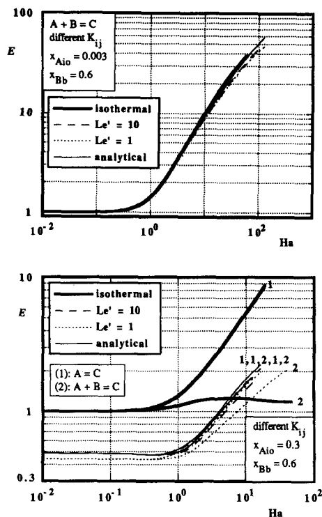
Fig. 7. Dimensionless absorption flux \mathcal{E} of component A obtained from the numerical model and the analytical expressions as a function of the Hatta number in case of the solubility, the binary mass transfer coefficients and the chemical reaction rate constant are temperature dependent: (a) second-order chemical reaction, different binary mass transfer coefficients and second composition regime; (b) first-order and second-order chemical reaction, different binary mass transfer coefficients and third composition regime. Parameter values are given in Table 1.
