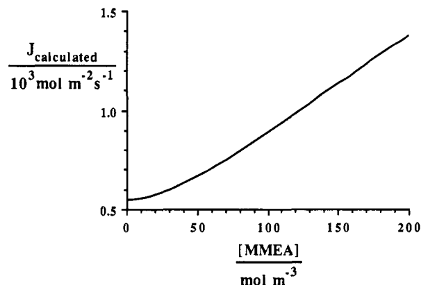
Figure 5. Calculated absorption fluxes for mixtures of MMEA and MDEA ( T = 303 K , [MDEA] + [MMEA] = 2599 \text{ mol m}^{-3} , [COS]_{g,int} = 16.2 \text{ mol m}^{-3} , [COS]_{L,tot} = 0 \text{ mol m}^{-3} , k_{L,COS} = 3.32 \times 10^{-5} \text{ m s}^{-1} ).
