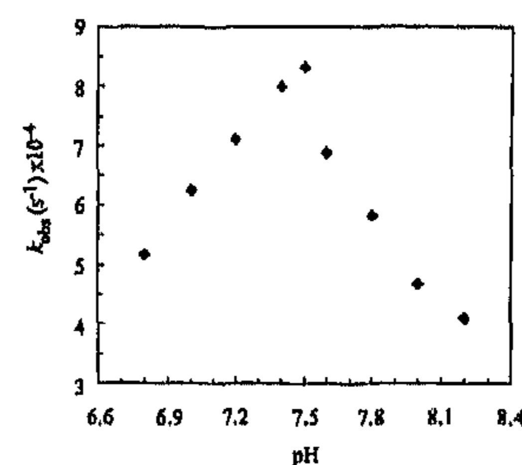
Figure 2. pH vs rate profile for transesterification of HPNP (0.19 mM) catalyzed by 1 (0.48 mM) in acetonitrile/20 mM HEPES 1:1 (v/v) at 25 °C.
