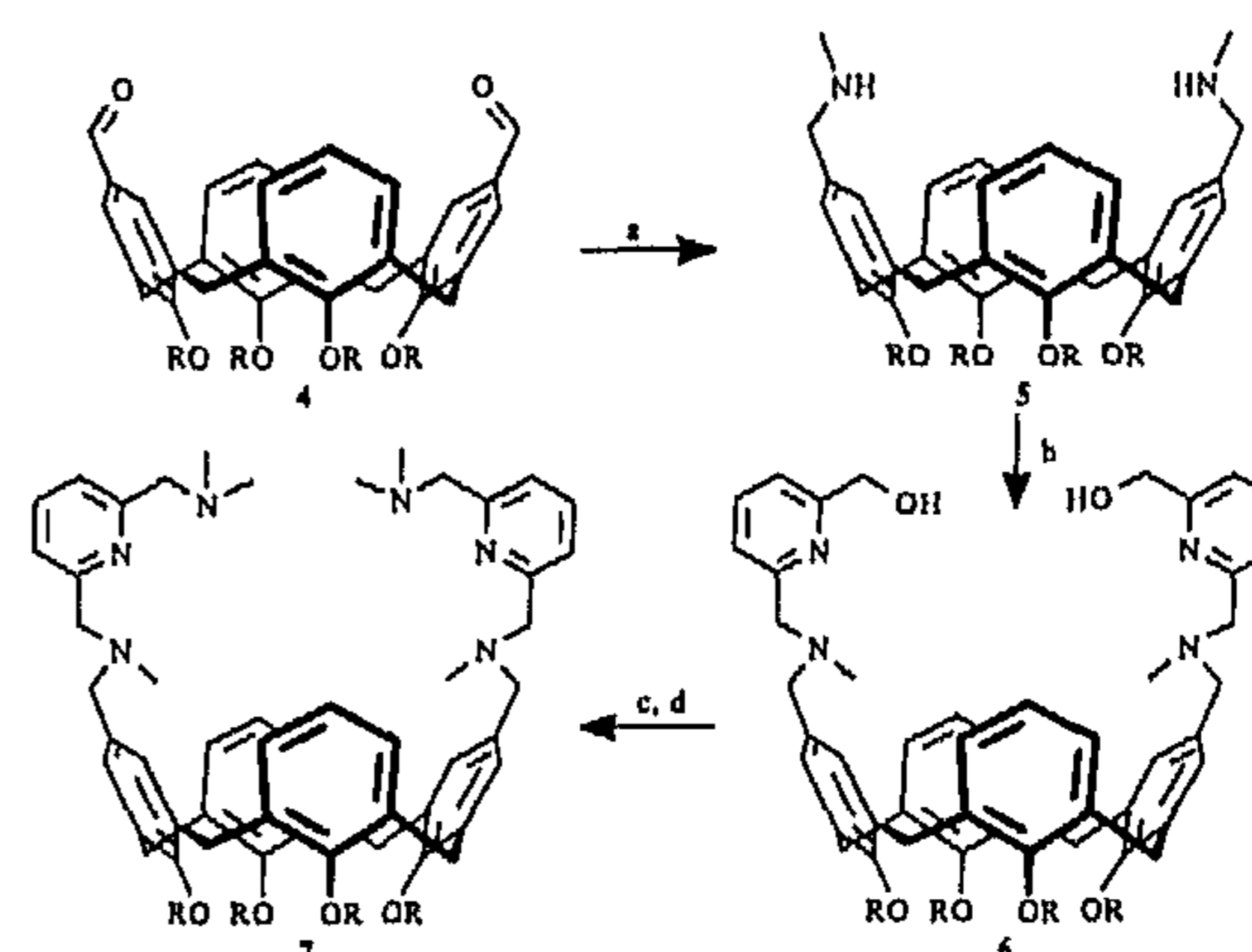
Scheme 1. Synthesis of a Calix[4]arene-Based Dimeric Ligand (R = CH 2 CH 2 OEt) a
