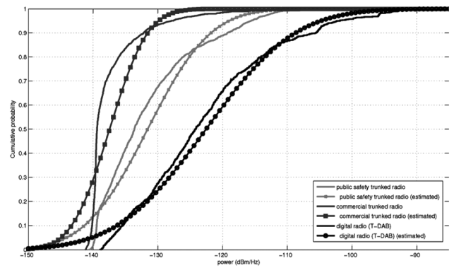
Fig. 4: CDFs of several radio networks based on the measurement data of Fig. 3.
