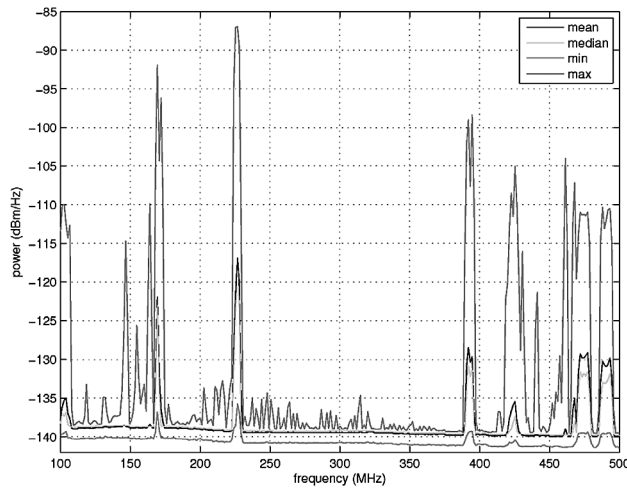
Fig. 3: The measured radio spectrum in Amsterdam.
