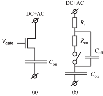
Fig. 5. (a) Schematic of a transistor in series with a capacitor. If sufficient gate bias V_{gate} is applied on the transistor, a channel will be formed between the source and the drain, connecting the capacitor to the circuit. (b) Loss model of the transistor-switched capacitor. If the switch is closed, R_{ON} will dominate the performance. If the switch is open, the OFF-capacitance C_{OFF} will dominate the minimum capacitance. The capacitance C is assumed to be an ideal capacitor, e.g., a low-loss MIM capacitor.
