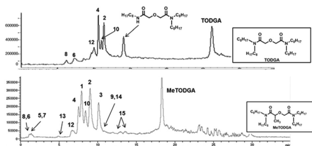
Fig. 7 HPLC-MS(APCI + ) chromatograms for TODGA and MeTODGA irradiated to 1000 kGy in acid pre-equilibrated TPH. Peak numbers correspond to compounds in Fig. 4.
