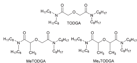
Fig. 1 Structures of TODGA, MeTODGA and Me 2 TODGA.
