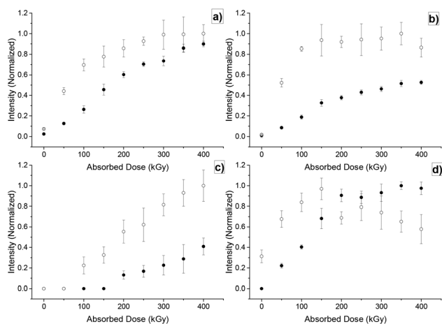
Fig. 9 Formation of compounds (a) 1 , (b) 19 , (c) 20 , and (d) 18 (Fig. 8) versus absorbed dose for the irradiation of 0.05 M MeTODGA in n -dodecane (solid squares), for pure organic samples, and for samples irradiated in the presence of 2.5 M HNO 3 (open squares). Intensities are normalized to the maximum detected signal for each compound.
