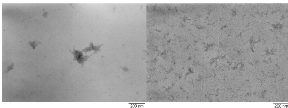
Figure 6. TEM view of jellified sols of zirconium n -propoxide modified with 1/2 mol equivalent of H_2dea without (left) and with (right) refluxing before hydrolysis.
