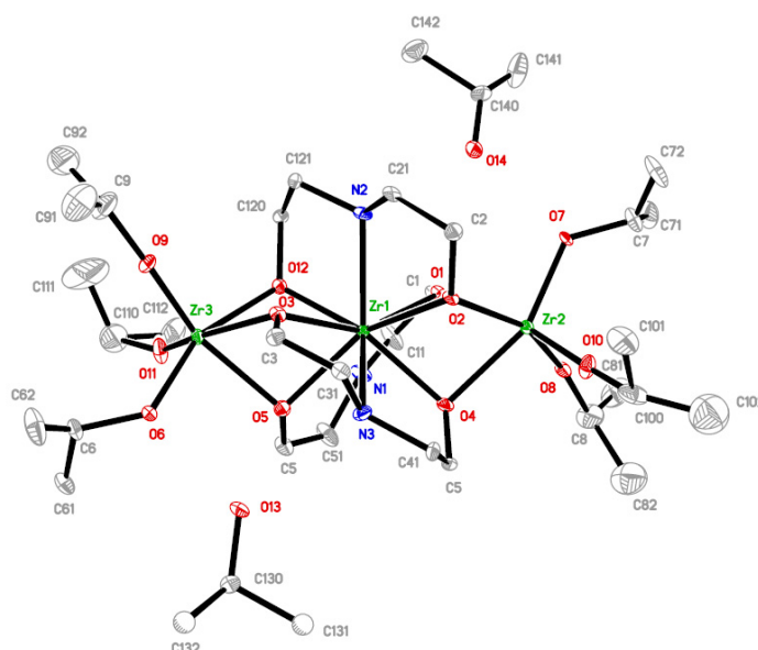
Figure 3. Molecular structure of \text{Zr}\{\eta^3\mu_2\text{-NH}(\text{C}_2\text{H}_4\text{O})_2\}_3[\text{Zr}(\text{O}^i\text{Pr})_3]_2(\text{}^i\text{PrOH})_2 ( 3 ).
