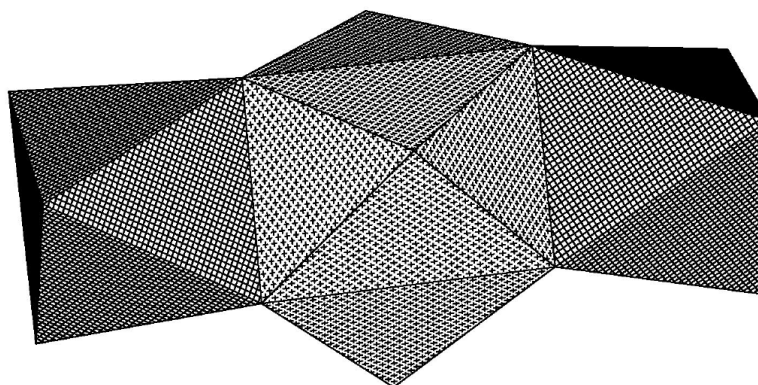
Figure 4. Polyhedral presentation of the molecular structure of 3 .
