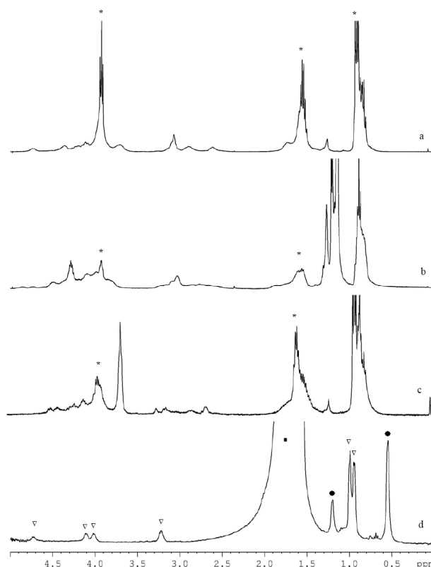
Figure 5. ^1\text{H} NMR spectra of the freshly prepared 1 (a) and 2 (b); and of crystals of 1 aged for 3 weeks at r.t. (c), and a fresh sample of 3 (d) in toluene as solvent. The signals assigned to the n -propoxide are marked with (*), to toluene and hexane with (■) and (●), and those assigned to 3 with (∇) respectively.
