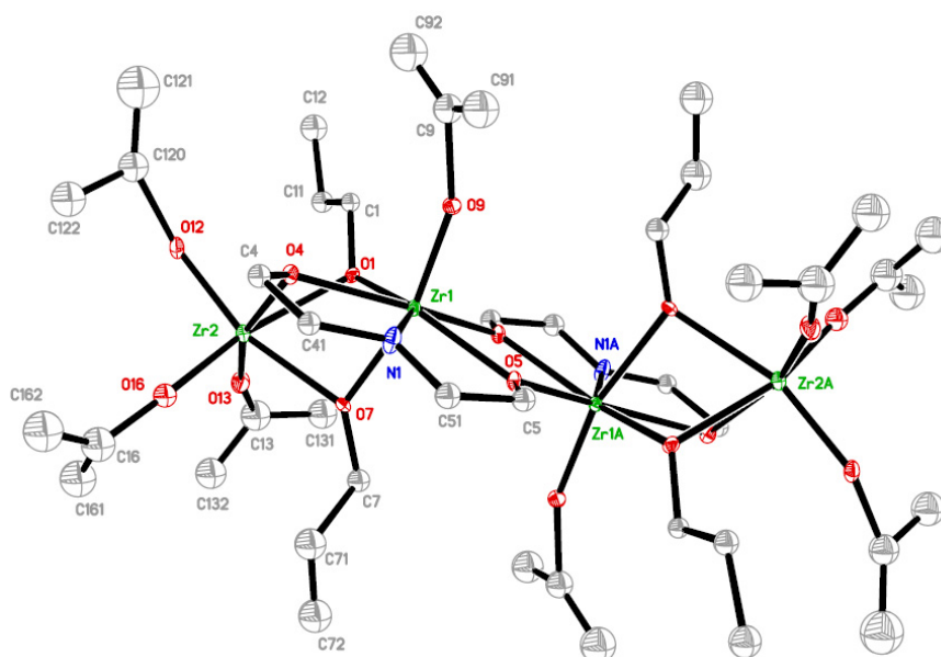
Figure 2. Molecular structure of [Zr 2 (O n Pr) 2 (O i Pr) 4 (OCH 2 CH 2 ) 2 NH] 2 ( 2 ).
