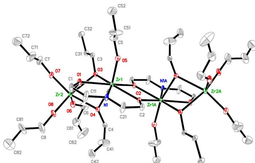
Figure 2. Molecular structure of [Zr 2 (O n Pr) 2 (O i Pr) 4 (OCH 2 CH 2 ) 2 NH] 2 ( 2 ).
