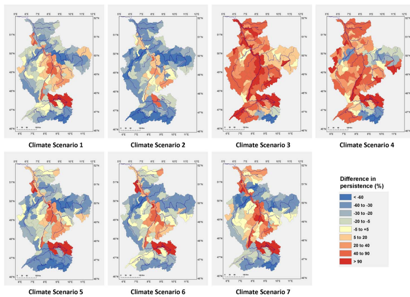
Fig. 4. Relative differences (%) * between low flow persistence estimated from simulated low flows using simulated inputs from seven climate scenarios for the reference period 1964–2007 (case 3) and simulated low flows using observed inputs for the same period (case 2). * (Based on simulated input – Based on observed input)/Based on observed input.
