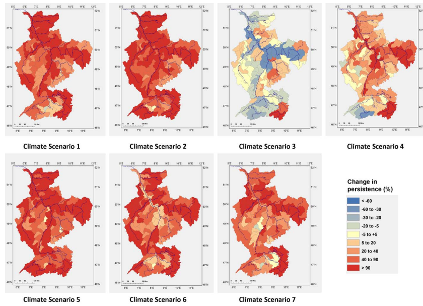
Fig. 7. Relative change (%)* in low flow persistence in 134 sub-catchments based on simulated low flows using simulated inputs from seven climate scenarios for the future period 2063–2098 (case 4) compared to simulated low flows using simulated inputs for the reference period 1964–2007 (case 3). * (Future period – Current period)/Current period.
