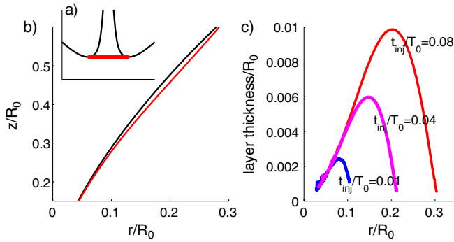
FIG. 5 (color online). A line of tracer particles is injected at the base of the jet at t_{\text{inj}}/T_0 = 0.08 (a). After advecting them backwards in time to the moment of pinch-off they form the border of a thin surface layer containing the liquid that eventually ends up in the jet (b). A corresponding movie is included as EPAPS_1 [22]. (c) The thickness of the layer that has gone into the jet at three different times.
