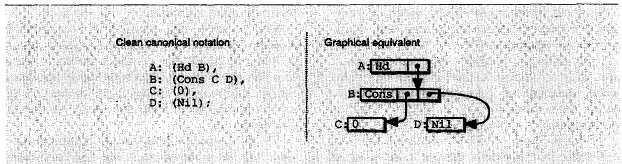
Fig. 1. Graph example.
