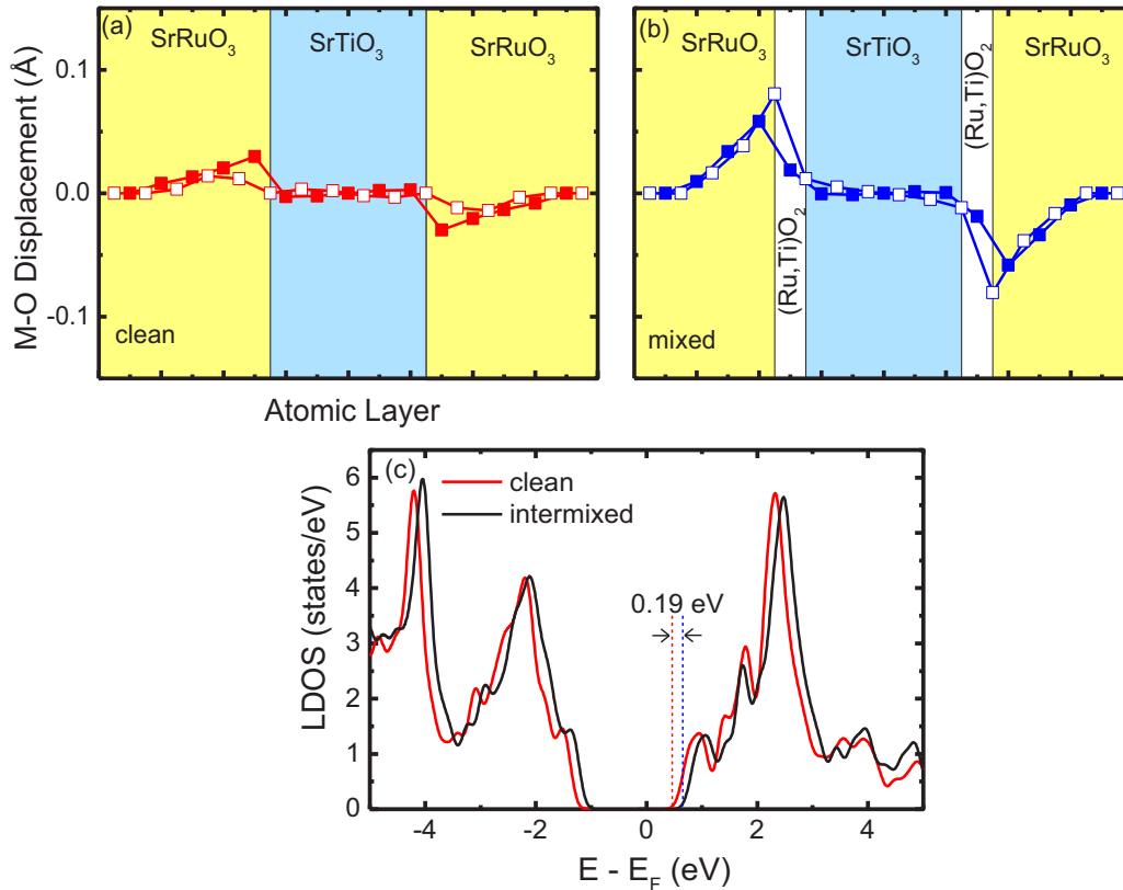
FIG. 5. Layer-by-layer metal-oxygen displacements for the two SrRuO 3 /SrTiO 3 supercells used to simulate the (a) T-Nb:STO and (b) S-Nb:STO interface. Solid symbols indicate the (Ru or Ti)O 2 displacements and the open symbols are for the SrO layers. (c) The local density of states in the center of the SrTiO 3 for both interface terminations. Vertical dashed lines indicate the position of the conduction-band minimum (CBM) with respect to the Fermi level, E_F .
