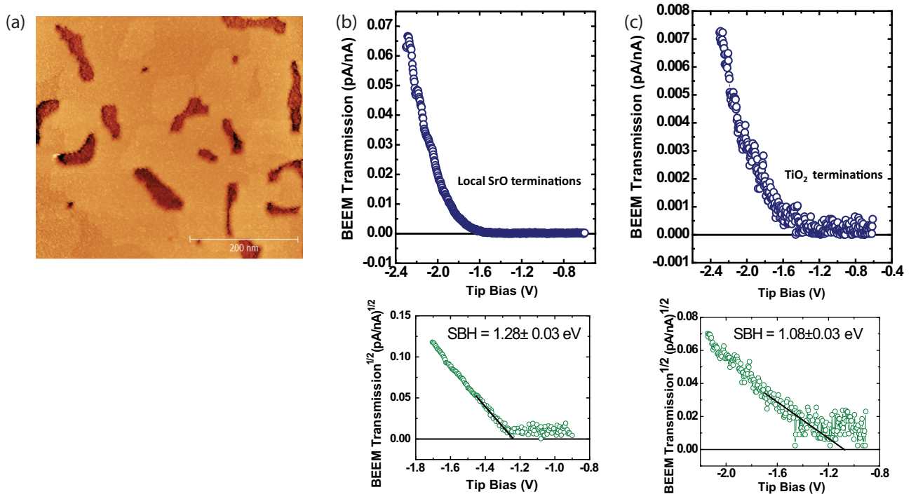
FIG. 3. (a) STM topography of 8 u.c. of SrRuO 3 grown on T-Nb:STO at V_{\text{tip}} = -1.4 V and I_{\text{tunnel}} = 4 nA. Occasional dark patches indicate thinner SrRuO 3 grown on SrO terminations of the substrate. (b) Corresponding BEEM spectra for tip placed in dark patches (trenches), i.e., on SrO terminations of the substrate. The extracted local SBH is represented below. (c) BEEM spectra for tip placed on TiO 2 terminated regions, i.e., on thicker SrRuO 3 growth. Corresponding local Schottky barrier height below.
