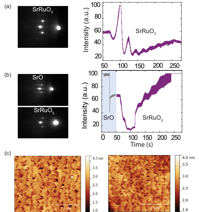
FIG. 1. Growth of 8 u.c. of SrRuO 3 on TiO 2 and SrO terminated substrates. (a) RHEED data for SrRuO 3 growth on nonengineered substrate T-Nb:STO. (b) RHEED data for the growth of a monolayer of SrO followed by 8 u.c. of SrRuO 3 . (c) AFM scan image of T-Nb:STO and S-Nb:STO.
