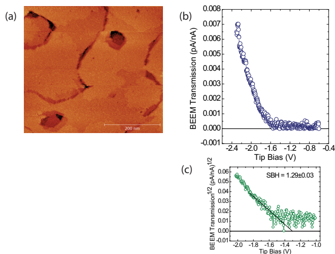
FIG. 4. (a) STM topography of 8 u.c. of SrRuO 3 grown on S-Nb:STO at V_{\text{tip}} = -1.4 V and I_{\text{tunnel}} = 4 nA. (b) Corresponding BEEM spectra through 8 u.c. of SrRuO 3 grown on S-Nb:STO. (c) The extracted local Schottky barrier height. Clearly, the local SBH matches with that extracted from SrRuO 3 grown inside the trenches of T-Nb:STO as shown in Fig. 3(b).
