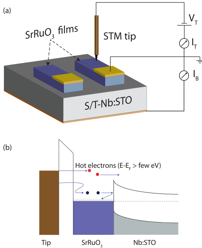
FIG. 2. (a) Fabrication of multiple SrRuO 3 devices grown on Nb:STO. Analyses were done on many different devices to understand the electronic behavior of the film-substrate interface. (b) Schematic diagram of BEEM, where the Pt-Ir STM tip injects hot electrons over the vacuum barrier into a thin metallic film of SrRuO 3 . The transmitted electrons that satisfy the energy and momentum criteria to overcome the SBH at the interface are collected in the Nb:STO semiconductor.
