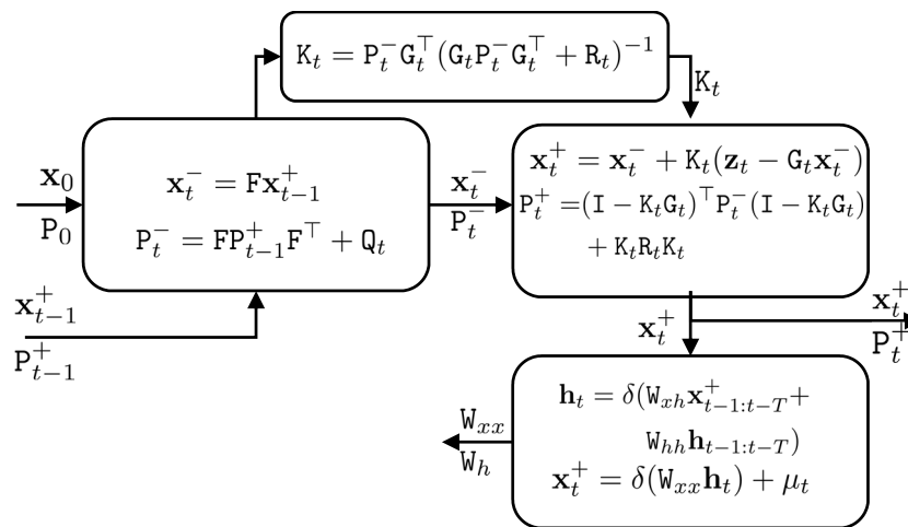
Figure 3. The deep Kalman filter procedure. The IMU modelling step (right-bottom) has been added to the Kalman filter. The modelling is accomplished in two steps: in the first step, the current latent vector is estimated based on previous latent and state vectors; and in the second step, the current state vector is estimated based on the current latent vector.
