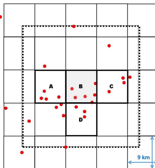
Fig. 1. Example of the SMAP L2SMP_E grid over a core validation site (Walnut Gulch). The solid black lines indicate the borders of the 9-km grid cells. The circles are the locations of in situ stations. The CVS 9-km grid cell is chosen (the heavier black line grid cell “B”) so that its actual contributing domain of 33-km (the dashed black line centered on grid cell “B”) best captures the data from the local network of stations.
