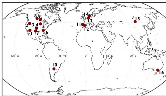
Fig. 2. Locations of the core validation sites (CVS) used in the study.
