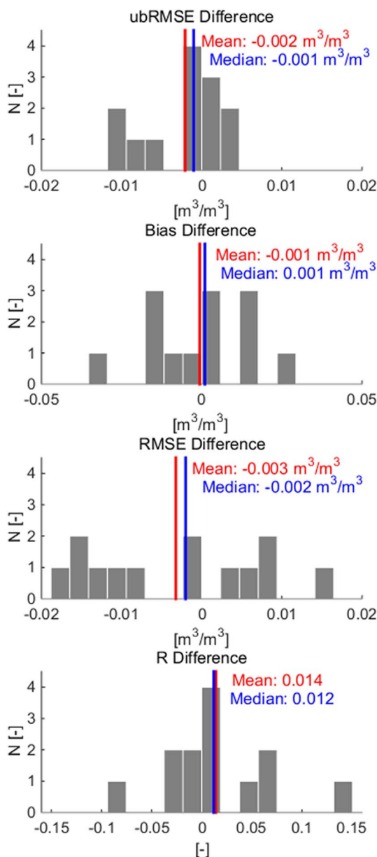
Fig. 3. Distribution of the differences between metrics obtained with 33-km grid cells and 9-km grid cells (33-km minus 9-km).
